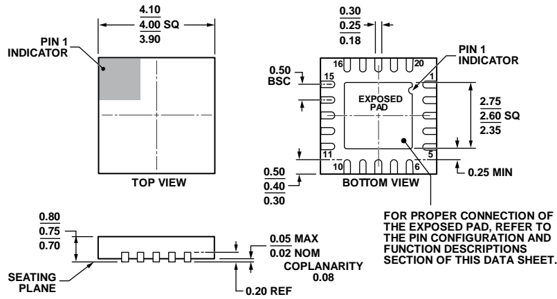
Figure 29. 20-Lead Lead Frame Chip Scale Package [LFCSP_WQ] 4 mm × 4 mm Body, Very Very Thin Quad (CP-20-8)
